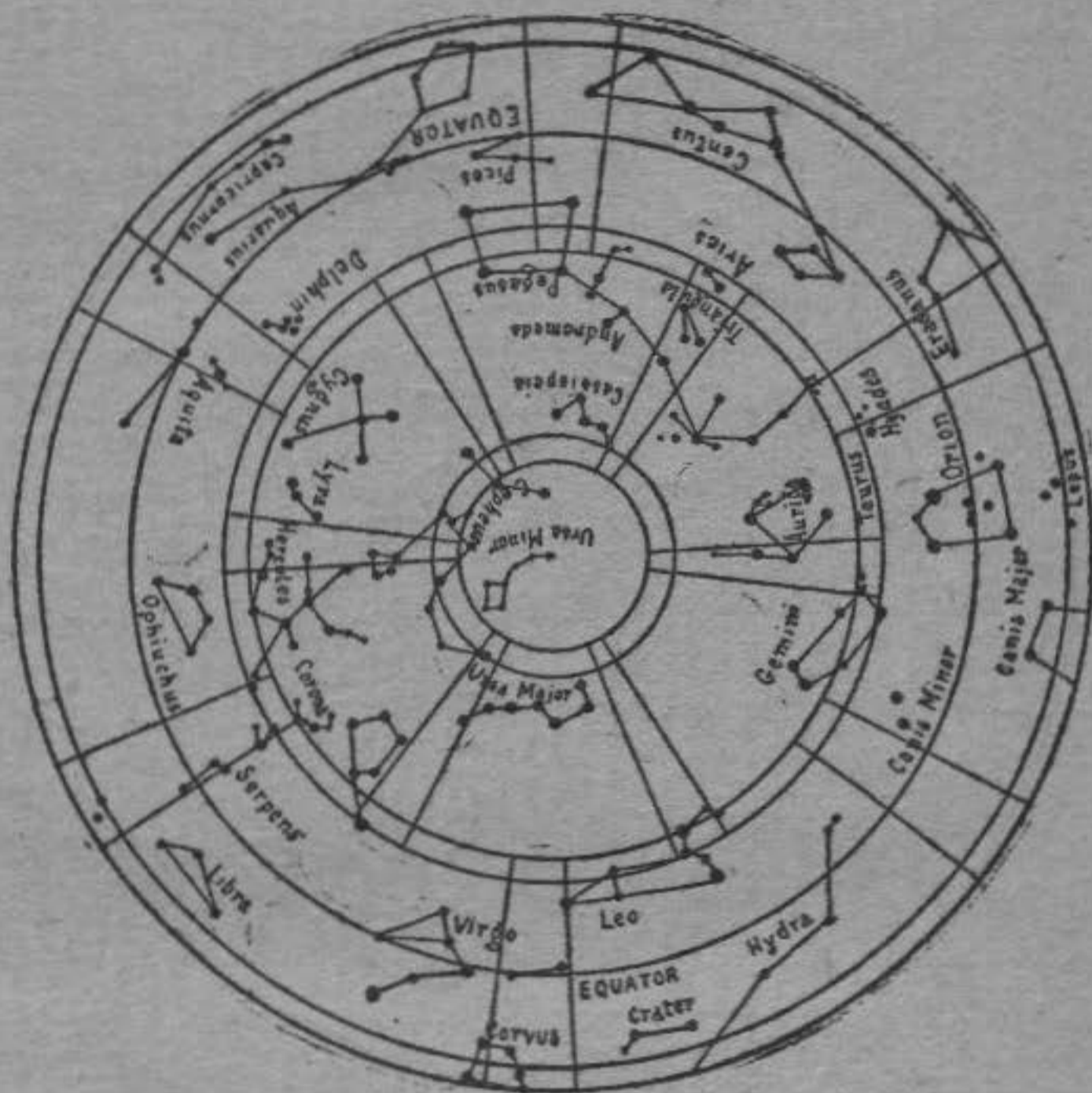
THE PRINCIPAL CONSTELLATIONS OF THE NORTHERN SKY.
