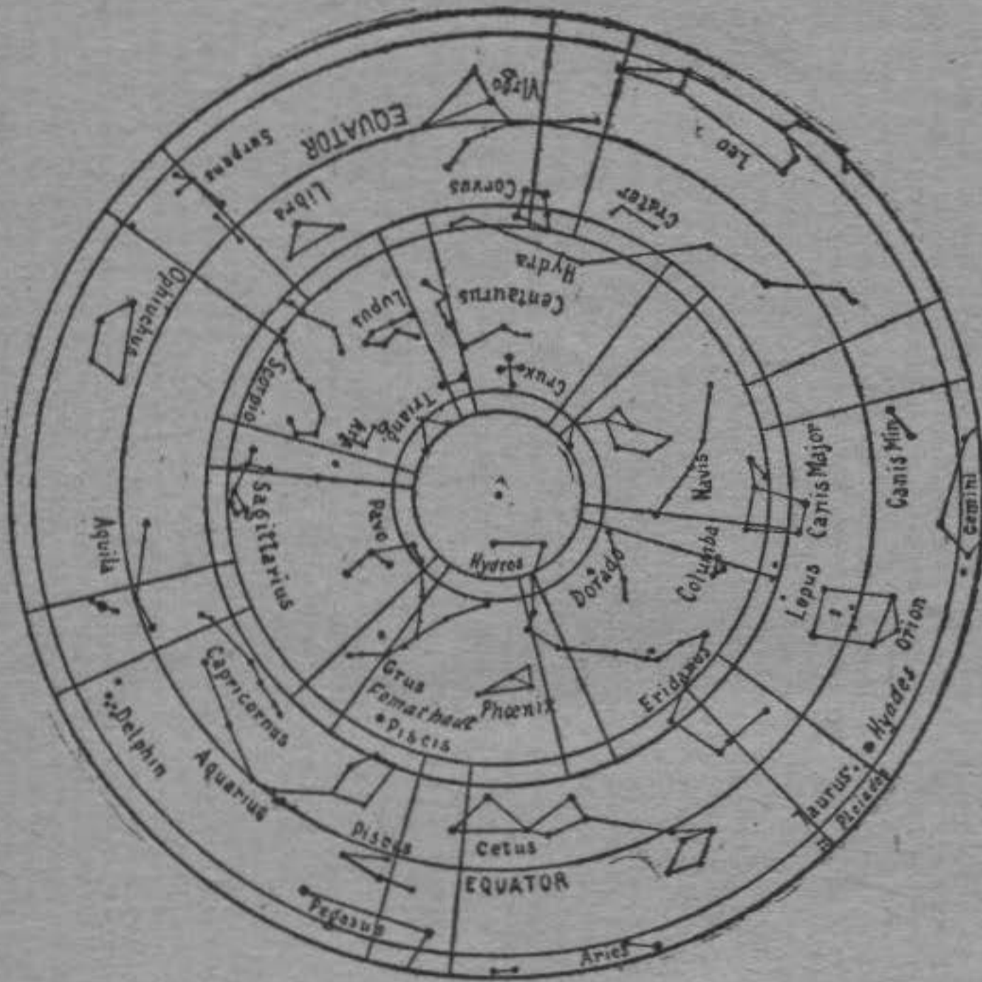
THE PRINCIPAL CONSTELLATIONS OF THE SOUTHERN SKY.
