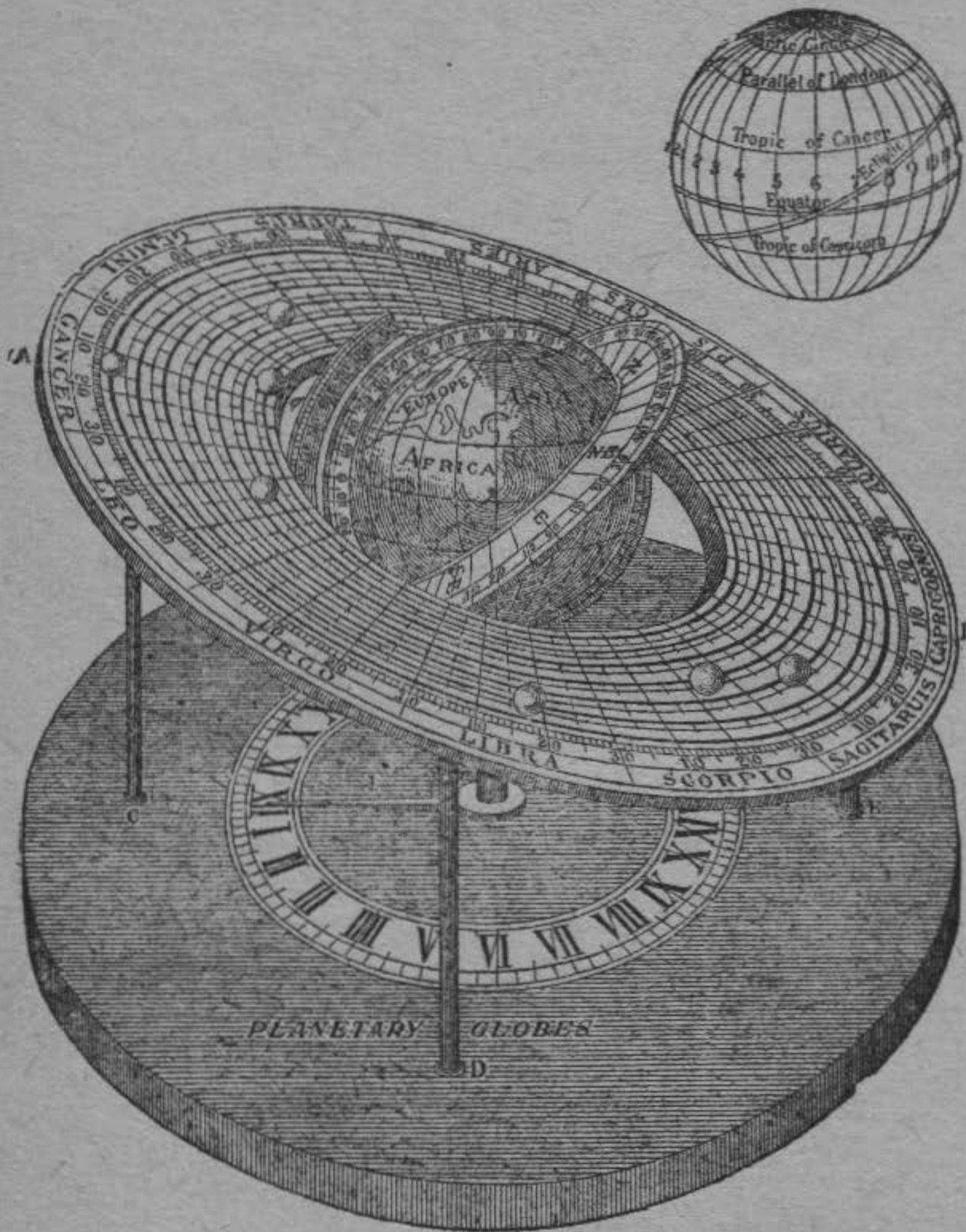
An ancient instrument demonstrating the distance of the planets from the earth and the plane of their paths. The smaller cut represents the earth, its zones, equator, etc.
